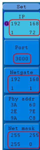
Fig.5-52 Set the network parameters of the oscilloscope
