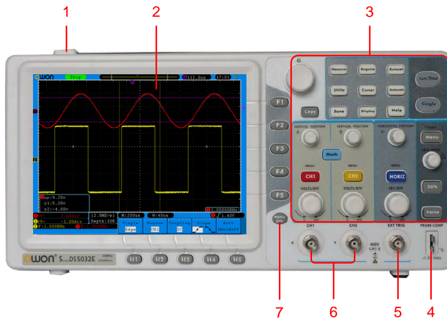
Fig. 4-1 Front panel
