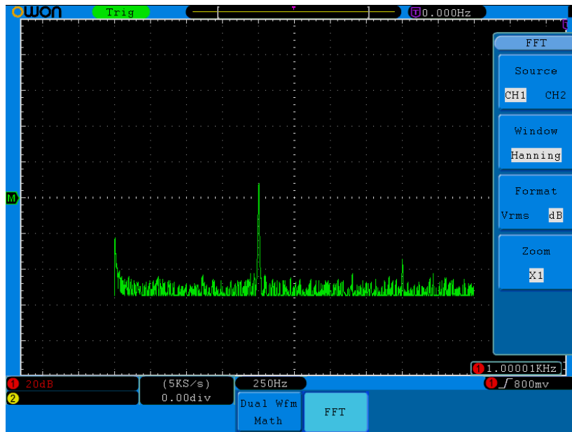
Fig.5-10 Hanning window
