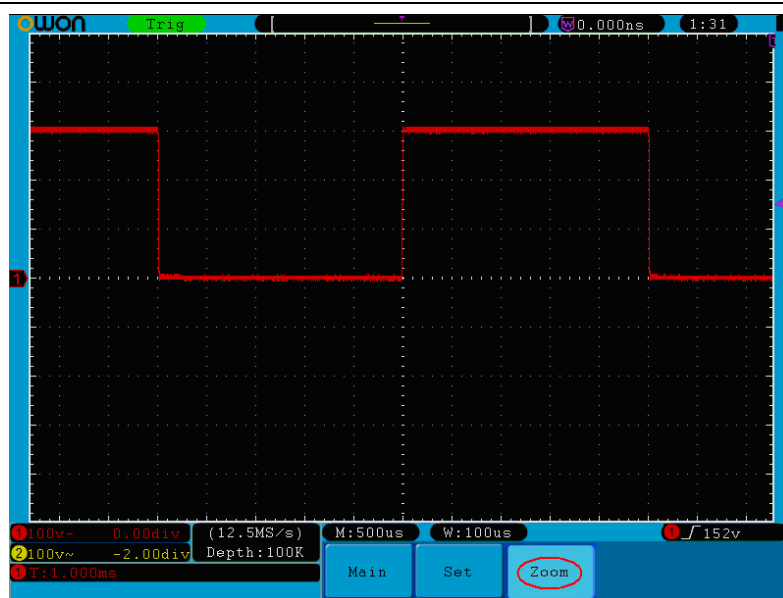
Fig. 5-16 Zoom Window
