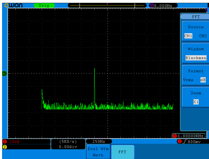
Fig.5-11. Blackman window
