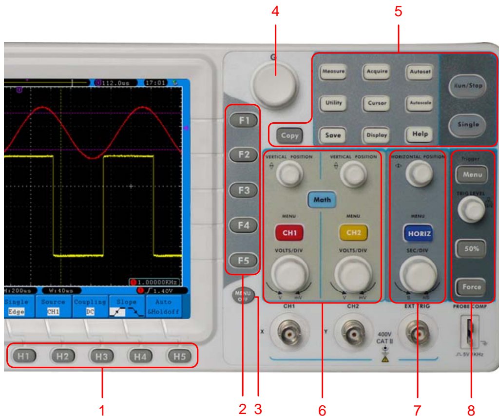
Fig. 4-4 Keys Overview
