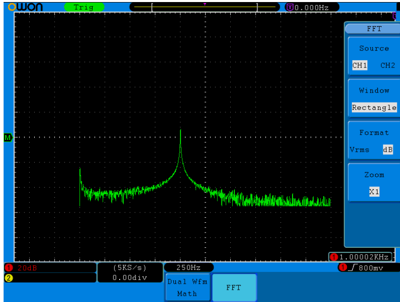
Fig.5-8. Rectangle window
